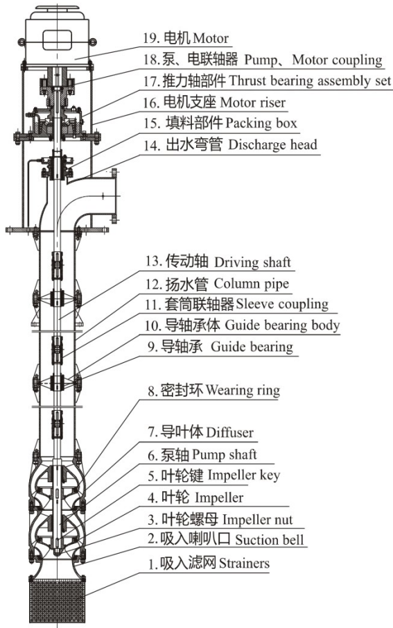
VTCF结构图(电机) Construction Drawing of VTCF(With Motor)
