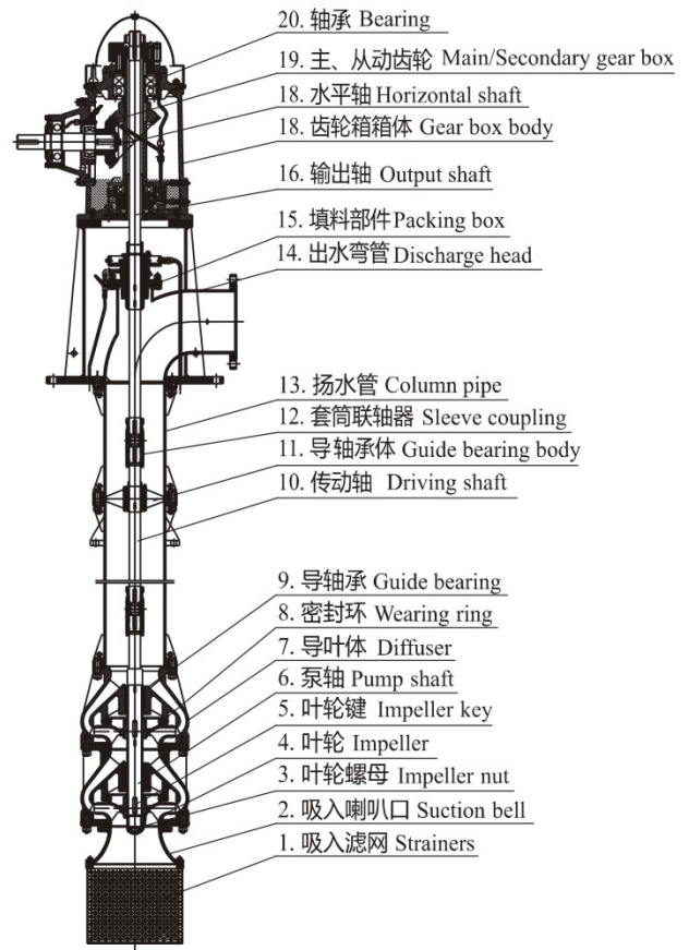
VTCF结构图(齿轮箱) Construction Drawing of VTCF(With Gear Box)
